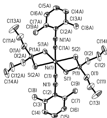
Figure 1. Perspective view of one of the two crystallographically independent but chemically equivalent molecules of [\text{Ni}\{\text{S}_2\text{P}(\text{OEt})_2\}_2(\text{CNXyl})_2] (2) , showing the atom numbering. The numbering of the second molecule can be obtained by adding 50 to the number in the label.
