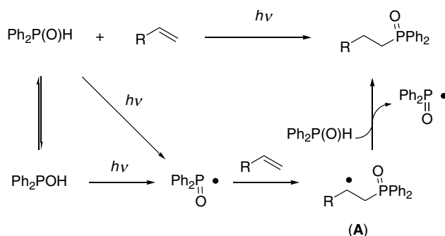
Scheme 2. A possible pathway of photoinduced hydrophosphinylation.
