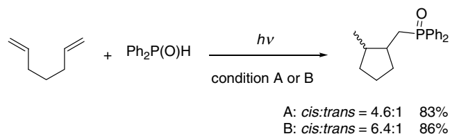
Photoinduced hydrophosphinylation of alkenes with \text{Ph}_2\text{P}(\text{O})\text{H} in the presence of pyridine
