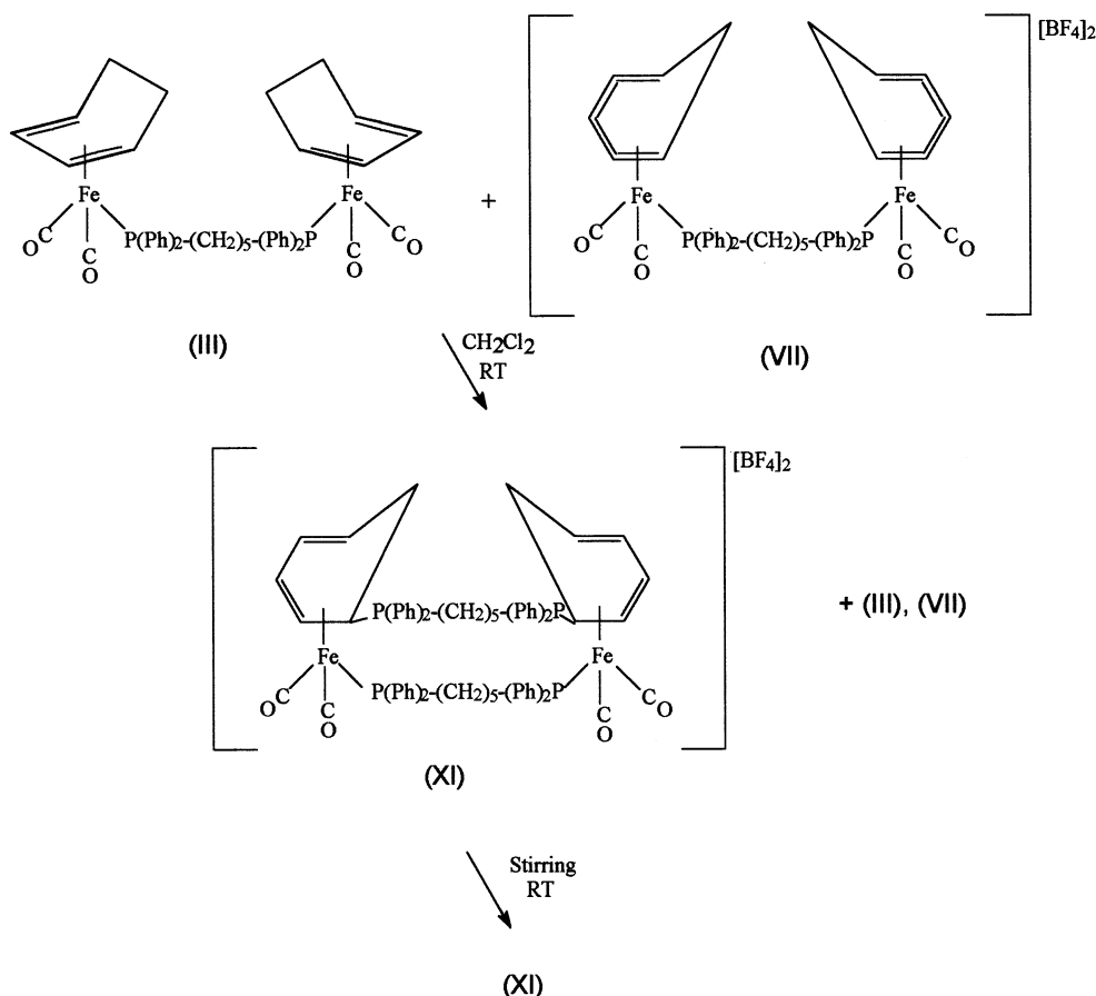
Scheme 2. Diphosphine transfer.
