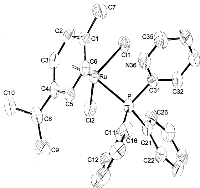
Fig. 2. Molecular structure of complex [\text{RuCl}_2(p\text{-cymene})(\text{PPh}_2\text{Py})] ( 3 ).
