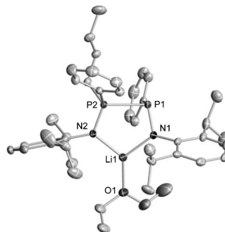
Fig. 1 Thermal ellipsoid plot of Li[DippNPhP-P(Bu^u)PhNDipp] \cdot OEt_2 ( 2 ). Hydrogen atoms have been omitted for clarity. Selected bond lengths (Å) and angles ( ^\circ ): P(1)–N(1) 1.6522(15), P(2)–N(2) 1.6065(15), P(1)–P(2) 2.2436(7), N(1)–Li(1) 1.939(3), N(2)–Li(1) 1.965(4), N(1)–P(1)–C(1) 108.90(8), N(1)–P(1)–P(2) 97.83(6), C(1)–P(1)–P(2) 93.04(6).
