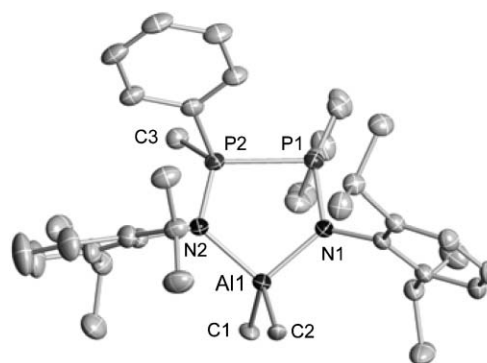
Fig. 2 Thermal ellipsoid plot of Al(Me)_2[DippNPhP-P(Me)PhNDipp] ( 3 ). Hydrogen atoms have been omitted for clarity. Selected bond lengths (Å) and angles ( ^\circ ): P(1)–N(1) 1.673(2), P(2)–N(2) 1.634(2), P(1)–P(2) 2.2367(11), N(1)–Al(1) 1.892(2), N(2)–Al(1) 1.929(2), N(1)–P(1)–C(4) 108.05(12), N(1)–P(1)–P(2) 95.36(8), C(4)–P(1)–P(2) 98.37(9).
