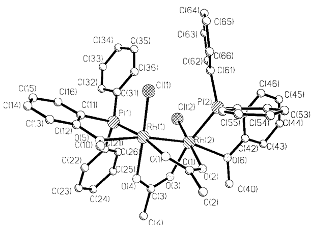
Fig. 2 Molecular view of [\text{Rh}_2(\mu\text{-O}_2\text{CCH}_3)_2(\text{Cl})_2\{\eta^2\text{-(}o\text{-CH}_3\text{C}_6\text{H}_4\text{)P(C}_6\text{H}_5\text{)}_2\}] 5 .
