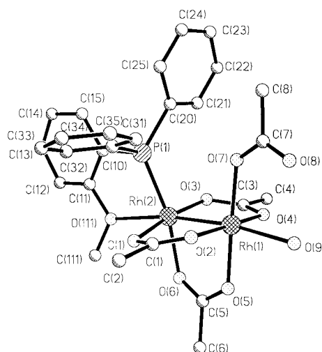
Fig. 3 Molecular view of [\text{Rh}_2(\mu\text{-O}_2\text{CCH}_3)_3(\text{O}_2\text{CCH}_3)\{\eta^2\text{-(}o\text{-CH}_3\text{OC}_6\text{H}_4\text{)P(C}_6\text{H}_5\text{)}_2\}] 1 . Atom O(9) corresponds to a water molecule.
