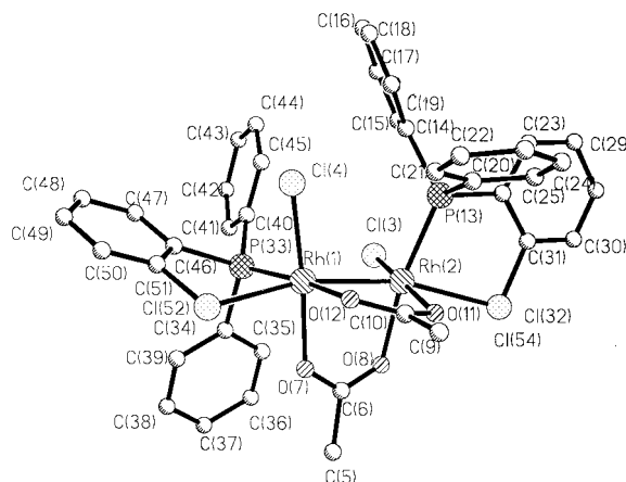
Fig. 1 Molecular view of [\text{Rh}_2(\mu\text{-O}_2\text{CCH}_3)_2(\text{Cl})_2\{\eta^2\text{-(o-ClC}_6\text{H}_4)\text{P(C}_6\text{H}_5)_2\}_2] , 4 .
