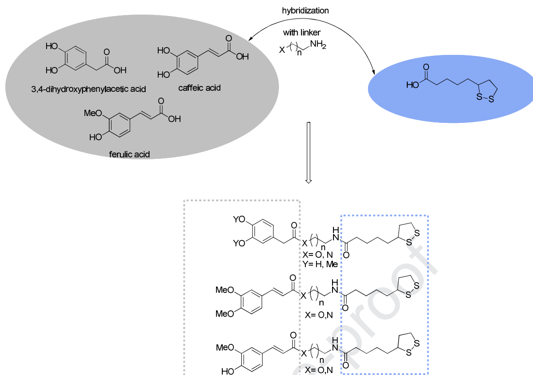
Figure 1. Design strategy towards phenolic acid – lipoic acid hybrids (SV1-13).
