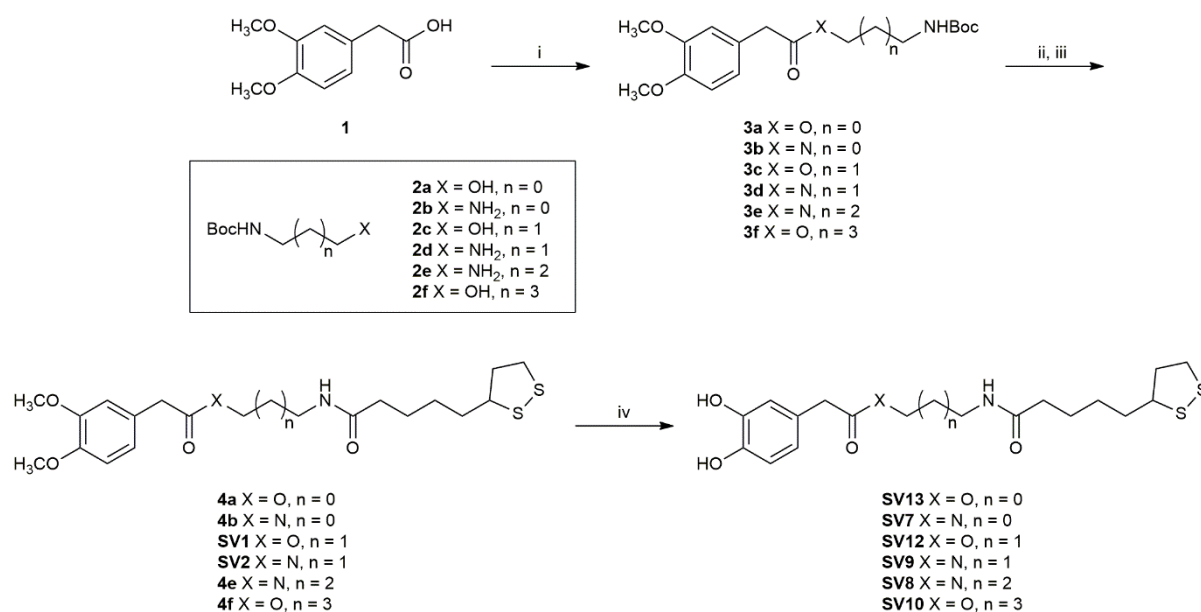
Scheme 1. Synthesis of SV1-2 , 8-10 , 12-13
