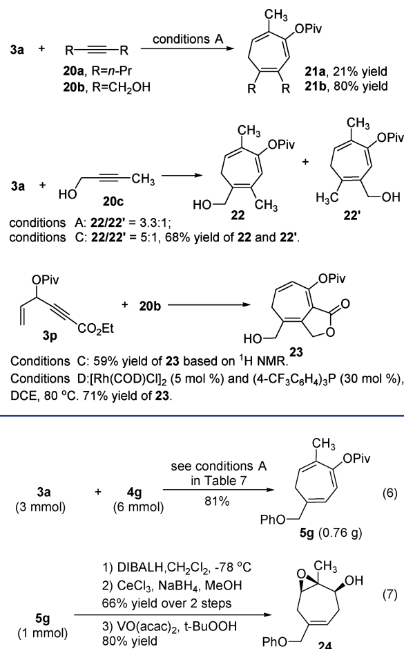
Scheme 3. Intermolecular Reaction of ACE 3a and Internal Alkynes (See Table 7 for Conditions A and C)
