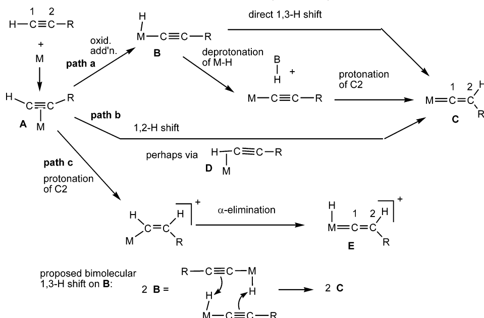
Scheme 1. Mechanistic Alternatives for Alkyne-to-Vinylidene Transformations
