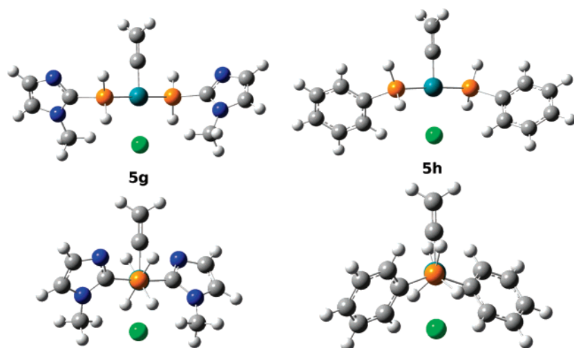
Figure 4. B3LYP/LANL2DZ lowest energy conformers of 5g and 5h . In each case the upper view is from a point perpendicular to the P–P axis, whereas the lower one is from a point on the P–P axis, showing the anti orientation of aromatic groups.
