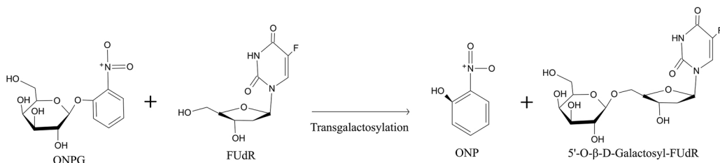
Scheme 1. Enzymatic galactosylation of FUDr.
