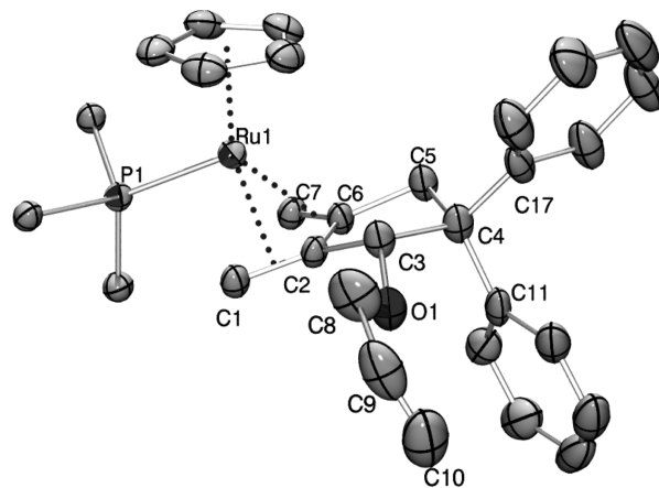
Figure 3. ORTEP drawing of the cationic ruthenium complex 9 . For clarity, aryl groups of the triphenylphosphine ligands on Ru except the ipso carbons and \text{PF}_6^- are omitted (thermal ellipsoid is set at the 50% probability level). Selected bond distances (Å) and angles (deg): Ru(1)–C(1), 2.210(4); Ru(1)–C(2), 2.196(4); Ru(1)–C(6), 2.193(4); Ru(1)–C(7), 2.207(4); C(1)–C(2), 1.408(5); C(2)–C(6), 1.416(5); C(6)–C(7), 1.395(5); C(1)–C(2)–C(6), 121.7(3); C(2)–C(6)–C(7), 122.1(3).
