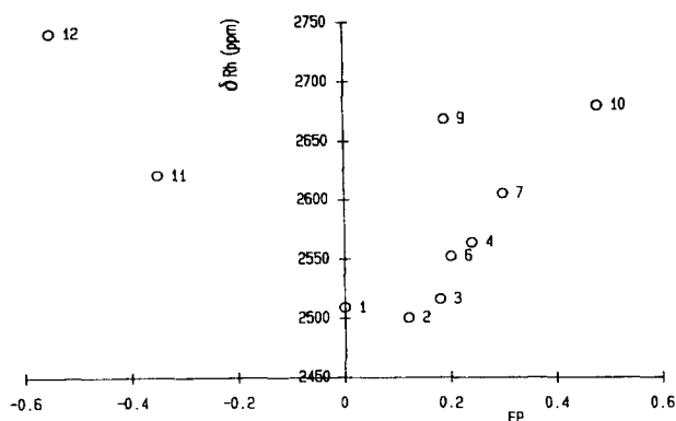
Fig. 2. ^{103}\text{Rh} chemical shifts in [\text{Rh}(\text{Hdmg})_2\text{Rpy}] vs. EP ( R = \text{Me} (1), \text{Et} (2), ^n\text{Pr} (3), ^i\text{Pr} (4), ^i\text{Bu} (6), ^s\text{Bu} (7), ^{nc}\text{Pent} (9), \text{adam} (10), \text{CH}_2\text{Cl} (11), \text{CH}_2\text{CF}_3 (12)).
