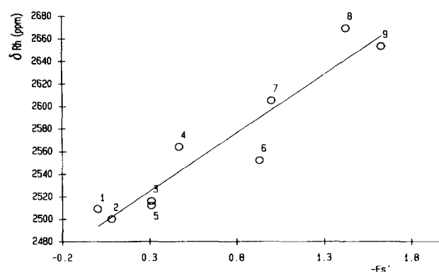
Fig. 4. ^{103}\text{Rh} chemical shifts in [\text{Rh}(\text{Hdmg})_2\text{Rpy}] vs. -Es' ( R = \text{Me} (1), \text{Et} (2), ^n\text{Pr} (3), ^i\text{Pr} (4), ^n\text{Bu} (5), ^i\text{Bu} (6), ^s\text{Bu} (7), ^t\text{Bu} (8), ^{nc}\text{Pent} (9)).
