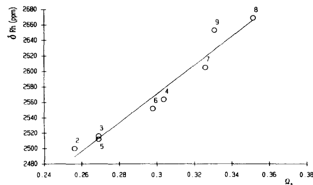
Fig. 5. ^{103}\text{Rh} chemical shifts in [\text{Rh}(\text{Hdmg})_2\text{Rpy}] vs. \Omega_s ( R = \text{Et} (2), ^n\text{Pr} (3), ^i\text{Pr} (4), ^n\text{Bu} (5), ^i\text{Bu} (6), ^s\text{Bu} (7), ^t\text{Bu} (8), ^{nc}\text{Pent} (9)).
