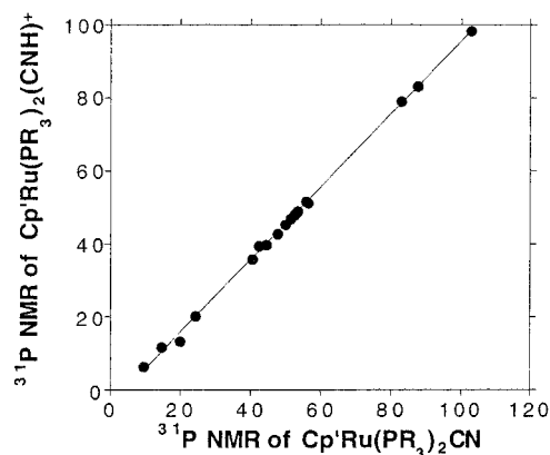
Figure 4. Correlation of the ^{31}\text{P} chemical shifts for \text{Cp}'\text{M}(\text{PR}_3)_2\text{CN} and for \text{Cp}'\text{M}(\text{PR}_3)_2(\text{CNH})^+ for 2CN , 5CN–9CN , 11CN–19CN , 23CN , 5*CN , 18*CN , and 19*CN and their protonated analogues.
