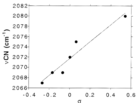
Figure 2. Correlation of the Hammett parameter ( \sigma ) and \nu(\text{CN}) for the \text{CpRu}[\text{P}(\text{aryl})_3]_2\text{CN} complexes, 8CN and 11CN–15CN .
