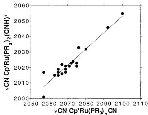
Figure 3. Correlation of \nu(\text{CN}) for \text{Cp}'\text{M}(\text{PR}_3)_2\text{CN} and for \text{Cp}'\text{M}(\text{PR}_3)_2(\text{CNH})^+ for 2CN , 5CN–8CN , 11CN–21CN , 23CN , 5*CN , 18*CN , and 19*CN and their protonated analogues.
