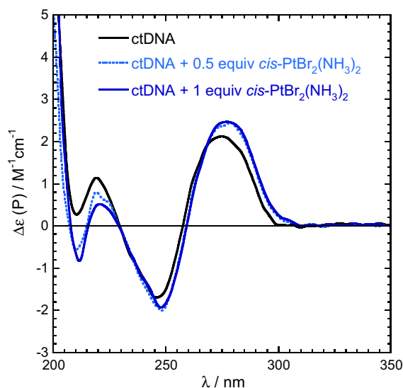
Fig. 4 CD spectra of ctDNA without and with cis -PtBr 2 (NH 3 ) 2 , 0.5 and 1 equiv, after 72 h incubation
