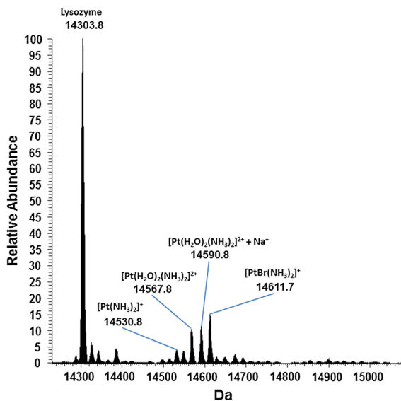
Fig. 3 Deconvoluted ESI MS spectra of lysozyme treated with 3 \times 10^{-4} mol L -1 of cis PtBr 2 recorded after 72 h of incubation at 37 °C, metal: protein ratio = 3:1; ammonium acetate buffer 20 mmol L -1 at pH 6.8
