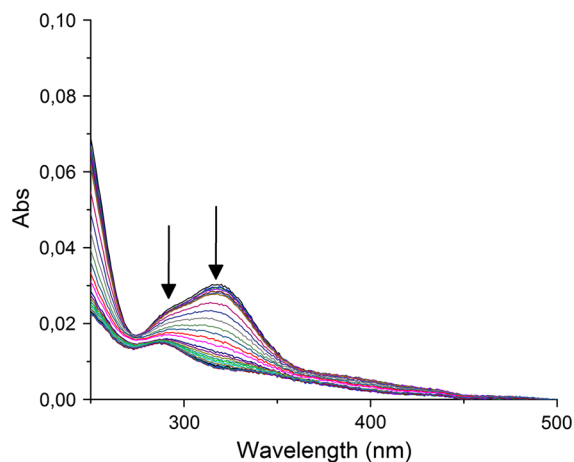
Fig. 2 Time course spectra of \text{cisPtBr}_2 10^{-4} M in 50 mM phosphate buffer recorded for 24 h, RT
