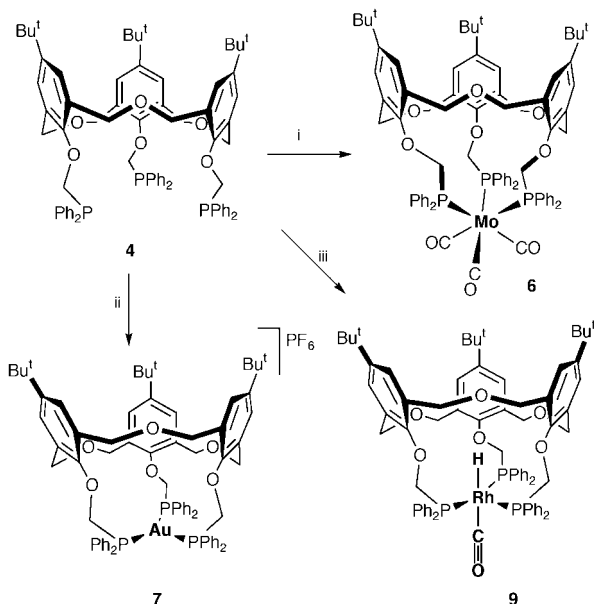
Scheme 1 Reagents and conditions: i, [Mo(CO) 3 (cycloheptatriene)], THF, reflux; ii, [Au(THT)(THF)]PF 6 , CH 2 Cl 2 ; iii, [Rh(acac)(CO) 2 ], 20 bar H 2 /CO, toluene, 70 °C.
