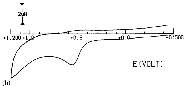
Fig. 3. Cyclic voltammetric responses recorded at a platinum electrode in CH 2 Cl 2 solutions containing (a) [(C 5 H 5 )Fe(C 5 H 4 ) 2 ]PPh (7 × 10 –4 M) and [NBu 4 ][ClO 4 ] (0.2 M), and (b) 6 (3 × 10 –4 M) and [NBu 4 ][PF 6 ] (0.2 M). Scan rate 0.2 V s –1 .
