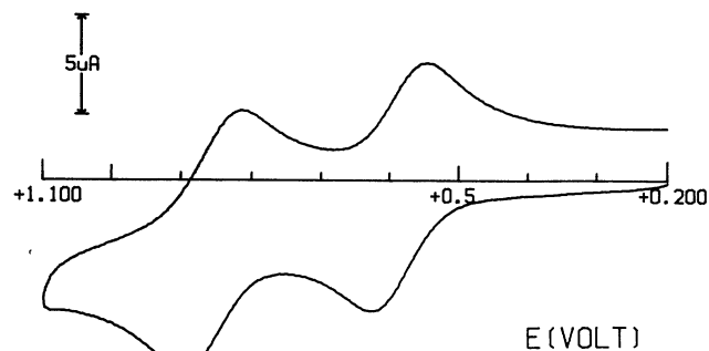
Fig. 4. Cyclic voltammetric response recorded at a platinum electrode in a CH 2 Cl 2 solution containing [Ru(L-6)Cl 2 ] (5 × 10 –4 M) and [NBu 3 ][PF 6 ] (0.2 M). Scan rate 0.2 V s –1 .
