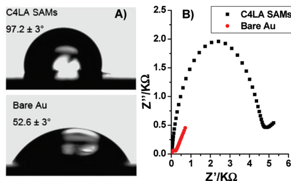
Figure 1. (A) Water-drop profiles on bare Au surface and C4LA /SAMs. (B) Impedance spectroscopy of 5.0 mM \text{Fe}(\text{CN})_6^{3-/4-} in 0.10 M \text{KNO}_3 aqueous solution on bare Au and C4LA SAMs electrode with the frequency ranging from 10 kHz to 1.0 kHz, scan rate: 0.10 v/s, indicating that C4LA successfully modified on gold surface.
