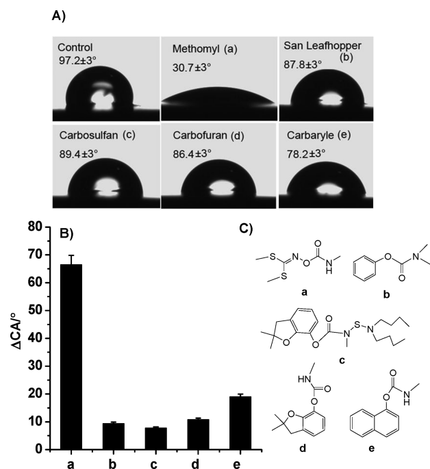
Figure 2. (A) CAs relationship images of C4LA SAMs with different guests: methomyl, san leafhopper, carbosulfan, carbofuran, carbaryl. (B) Contact angle variation ( \Delta CA = CA_{\text{control}} - CA ) histogram of C4LA SAMs in the presence of different carbamates, indicating that the selectively wettability responsive of C4LA toward methomyl. (C) Structure of the five guests.
