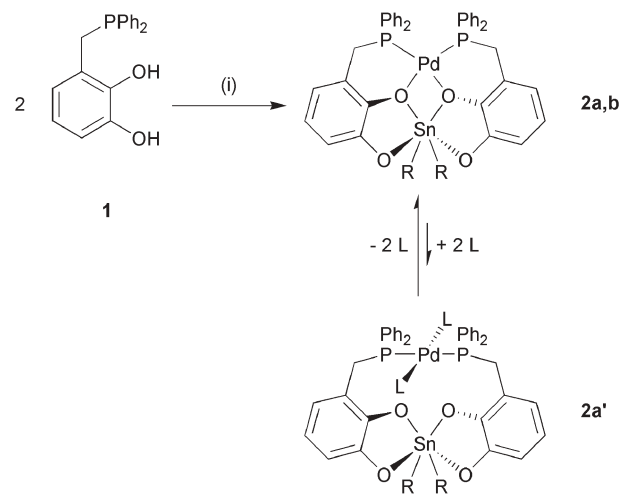
Scheme 2 Molecular bimetallic chelate complexes by self-assembly. R = Cl ( 2a ), Me ( 2b ); L = solvent (DMF or formamide). Reagents and conditions: (i) 1 equiv. R 2 SnCl 2 , 1 equiv. [(cyclooctadiene)PdCl 2 ], DMF–NEt 3 .
