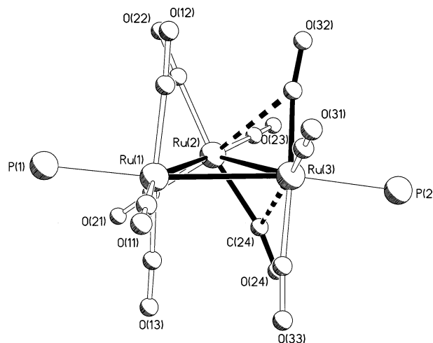
Fig. 2. A diagram of the molecular structure of complex 3 showing the orientations of the carbonyls with respect to the Ru_3 plane.
