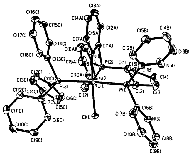
Figure 5. ORTEP representation of mer -RuCl 2 ( P,P,N -d(py)pcp)(PPh 3 ) ( 7a ) (50% probability ellipsoids).
