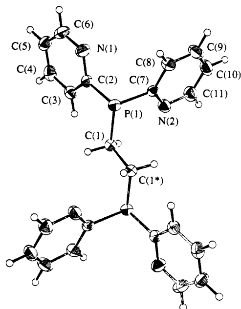
Figure 2. ORTEP representation of d(py)pe. Thermal ellipsoids for non-hydrogen atoms are drawn at 30% probability.
