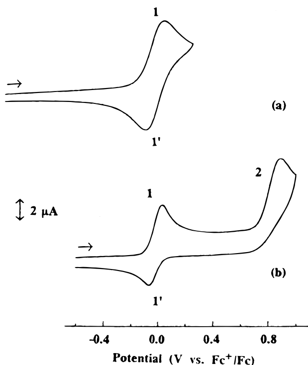
Figure 1. (a) Oxidative cyclic voltammogram recorded at a glassy carbon macrodisk electrode (scan rate 200 mV s -1 ) at 20 °C for a 1.0 mM solution of cis -Mn(CO) 2 (η 3 -P 3 )Cl in dichloromethane (0.1 M NBu 4 -NPF 6 ). (b) Voltammogram for similar conditions over an extended potential range.
