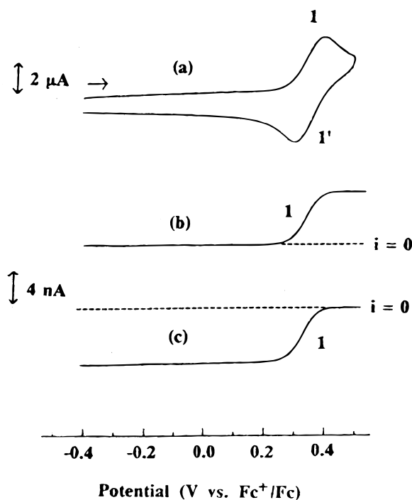
Figure 2. (a) Oxidative cyclic voltammogram recorded at a glassy carbon macrodisk electrode (scan rate 200 mV s -1 ) at 20 °C for a 1.0 mM solution of cis -Re(CO) 2 ( \eta^3 -P 3 )Cl in dichloromethane (0.1 M Bu 4 NPF 6 ). (b) Near-steady-state voltammogram (scan rate 10 mV s -1 ) recorded at a platinum microdisk electrode (radius 12.5 \mu m) at 20 °C for a 1.0 mM solution of cis -Re(CO) 2 ( \eta^3 -P 3 )Cl in dichloromethane (0.4 M Bu 4 NPF 6 ) before electrolysis. (c) Near-steady-state voltammogram of the same solution after subsequent exhaustive oxidative electrolysis.
