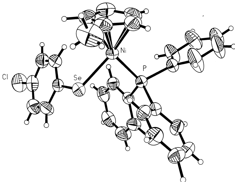
Fig. 2. ORTEP plot for \text{CpNi}(\text{PPh}_3)(\text{SeC}_6\text{H}_4\text{Cl-4}) .
