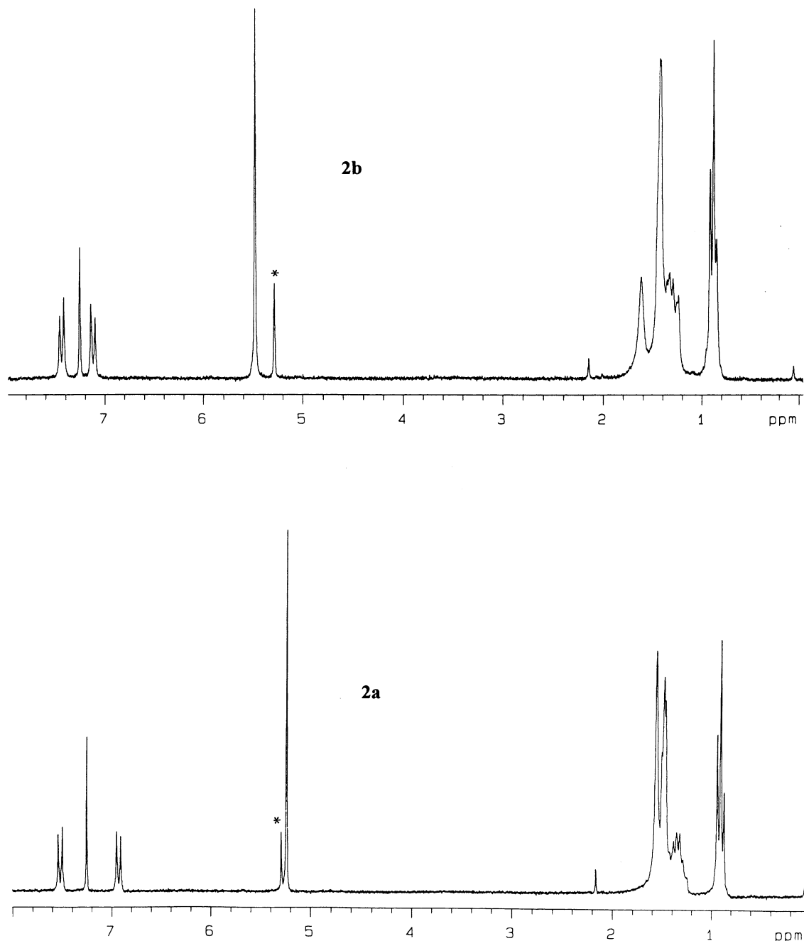
Fig. 3. ^1\text{H} -NMR spectra of \text{CpNi}(\text{PBU}_3)(\text{SC}_6\text{H}_4\text{Cl-4}) ( 2a ) and its \text{SO}_2 adduct ( 2b ). * Represents residual \text{CH}_2\text{Cl}_2 in each of the complexes.
