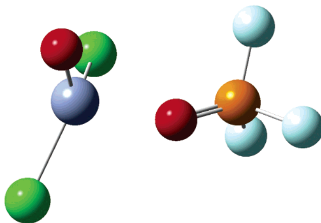
Figure 4. Representation of the \text{Cl}_2\text{CrO}-\text{OPF}_3 complex, calculated at the B3LYP/6-311++G(d,2p) level.
