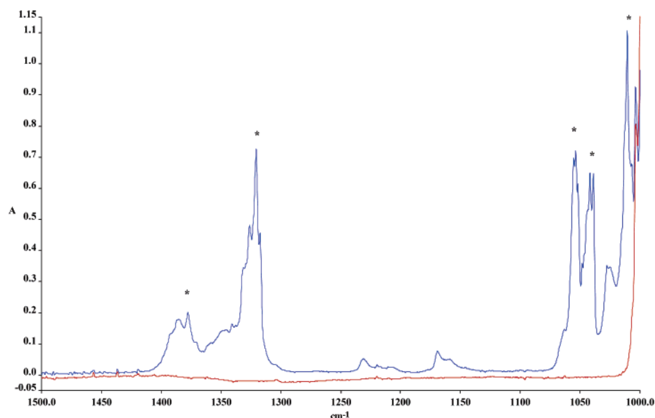
Figure 1. Infrared spectra before (lower) and after (upper) irradiation of argon matrices formed by the twin-jet deposition of samples of \text{Ar}/\text{PF}_3 and \text{Ar}/\text{CrCl}_2\text{O}_2 . The band marked with an asterisk denotes the major product bands.
