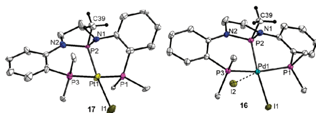
Figure 4. Displacement ellipsoid (50%) representation of 16 and 17 . For clarity, all hydrogen atom with the exception of those on the NHP-bound Me group have been omitted. Solvate molecules and PF_6^- counterions ( 17 ) have also been omitted. Relevant interatomic distances (Å) and angles (deg): 17 : P2–Pt, 2.228(3); Pt–P3, 2.311(4); Pt–P1, 2.322(4); P2–C39, 1.810(12); Pt–I1, 2.5961(8); I1–Pt–P2, 170.07(10); P3–Pt–P1, 173.45(11); Pt–P2–C39, 117.1(4). 16 : P2–Pd, 2.1984(5); Pd–P3, 2.3079(6); Pd–P1, 2.3051(6); P2–C39, 1.800(2); Pd–I1, 2.6617(2); Pd–I2, 3.1464(2); I1–Pd–P2, 170.590(16); P3–Pd–P1, 163.11(2); I1–Pd–I2, 105.726(7); Pd–P2–C39, 114.16(8).
