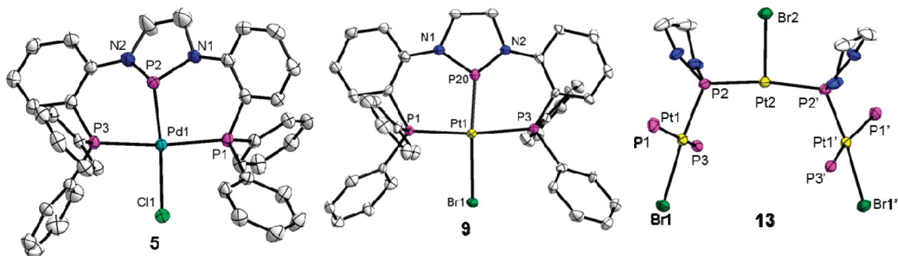
Figure 3. Displacement ellipsoid (50%) representation of 5, 9, and 13. For clarity, all hydrogen atoms and solvate molecules have been omitted. In the case of 13, aryl rings have also been omitted to reveal the core structure. The Pt-hydride ligand in 13 was not located crystallographically, and its position, therefore, is geometrically inferred. Relevant interatomic distances (Å) and angles (deg): 5: P2–Pd, 2.2424(13); P1–Pd, 2.3151(11); P3–Pd, 2.3098(11); Cl1–Pd, 2.4530(11); P1–Pd–P2, 90.528(48); P2–Pd–P3, 81.563(48); P1–Pd–Cl1, 94.035(42); P3–Pd–Cl1, 93.020(42); P1–Pd–P3, 170.959(38); P3–Pd–Cl1, 169.080(51). 9: P2–Pt, 2.2446(11); P1–Pt, 2.2901(19); P3–Pt, 2.2931(19); Br1–Pt, 2.5430(3); N1–Pt–N2, 89.055(168); P1–Pt–P2, 83.197(45); P2–Pt–P3, 90.224(45); P1–Pt–Br1, 93.856(31); P3–Pt–Br1, 93.434(30); P1–Pt–P3, 172.561(50); P2–Pt–Br1, 163.726(28). 13: P2–Pt1, 2.2111(11); P2–Pt2, 2.2756(11); P1–Pt1, 2.2903(13); P3–Pt1, 2.2906(11); Br1–Pt1, 2.5341(4); Br2–Pt2, 2.5432(7); P1–Pt1–P2, 88.822(44); P2–Pt1–P3, 88.774(41); P1–Pt1–Br1, 94.200(32); P3–Pt1–Br1, 89.599(27); P1–Pt1–P3, 163.935(42); P2–Pt1–Br1, 174.398(29); P2–Pt2–Br2, 94.352(25).
