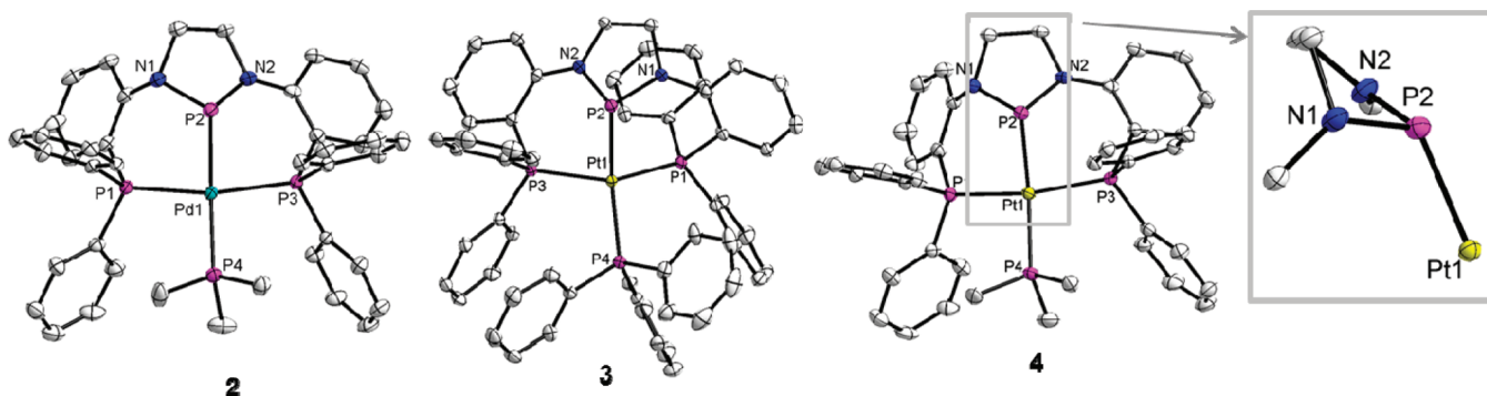
Figure 2. Displacement ellipsoid (50%) representation of 2 , 3 , and 4 . For clarity, all hydrogen atoms, \text{PF}_6^- counteranions, and solvate molecules have been omitted. Relevant interatomic distances (Å) and angles (deg): 2 : Pd–P2, 2.2535(6); Pd–P1, 2.3099(5); Pd–P3, 2.3384(5); Pd–P4, 2.4148(5); P1–Pd–P2, 86.128(23); P2–Pd–P3, 83.307(23); P3–Pd–P4, 97.750(22); P1–Pd–P4, 98.041(22); P1–Pd–P3, 161.993(19); P2–Pd–P4, 154.619(20). 3 : P2–Pt, 2.2600(7); P1–Pt, 2.3137(7); P3–Pt, 2.3190(6); P4–Pt, 2.3787(6); P1–Pt–P2, 86.081(23); P2–Pt–P3, 81.367(23); P3–Pt–P4, 102.287(21); P1–Pt–P4, 103.973(21); P1–Pt–P3, 147.173(22); P2–Pt–P4, 149.086(22). 4 : P2–Pt, 2.2606(9); P1–Pt, 2.3025(10); P3–Pt, 2.3123(11); P4–Pt, 2.367(1); P1–Pt–P2, 87.418(51); P2–Pt–P3, 84.453(50); P3–Pt–P4, 96.573(44); P1–Pt–P4, 96.912(44); P1–Pt–P3, 163.388(37); P2–Pt–P4, 154.962(33).
