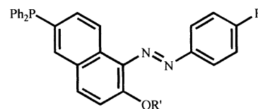
Fig. 1. Azo-containing phosphines \text{L} . \text{R}' = \text{H} , \text{R} = \text{Me} ( I ), \text{NMe}_2 ( II ), \text{NO}_2 ( III ); \text{R}' = \text{C(O)Me} , \text{R} = \text{Me} ( IV ), \text{NMe}_2 ( V ).
