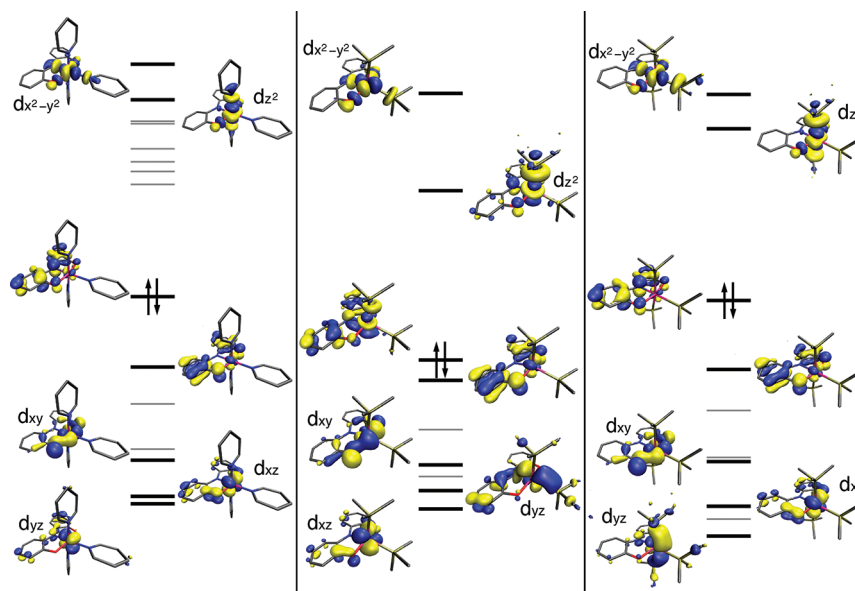
Figure 8. Calculated frontier molecular orbital diagrams displaying Kohn–Sham orbitals for 1 (left), 2a (center), and 3a (right). For each compound, the HOMO is designated with an electron pair. For clarity, only the HOMO, HOMO-1, and primarily d-based orbitals are illustrated.
