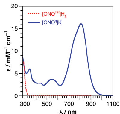
Figure 1. UV–vis absorption spectra of [\text{ONO}^{\text{cat}}]\text{H}_3 and [\text{ONO}^q]\text{K} acquired in \text{C}_6\text{H}_6 at 298 K.
