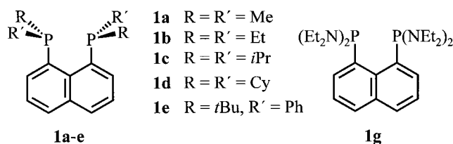
SCHEME 1 1,8-Bis(phosphino)naphthalenes.
