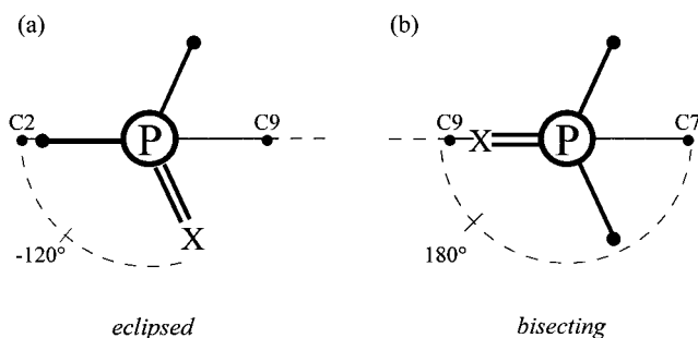
SCHEME 6 Idealized eclipsed (a) and bisecting (b) conformations of 1,8-bis(phosphinyl)naphthalenes. Numerical values are pseudo torsion angles (see text).
