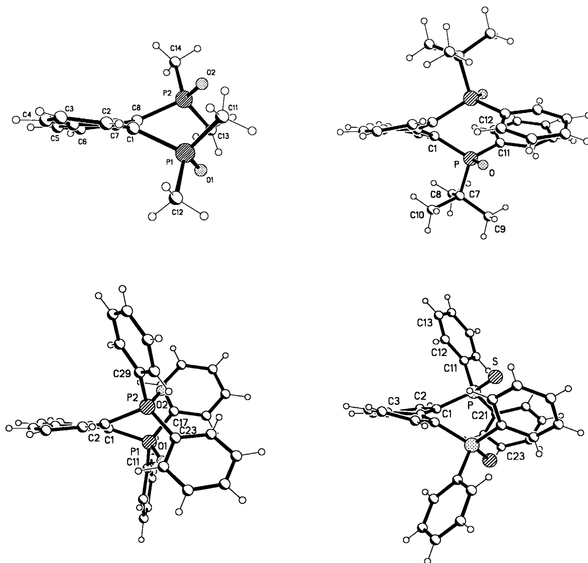
FIGURE 2 Molecular structures of 2a , ( S,S )- 2e , 2f , and 3f viewed along the C2...C9...C7 axis to illustrate the amount of out-of-plane displacement of the P(X)R 2 groups (X = O, S).
