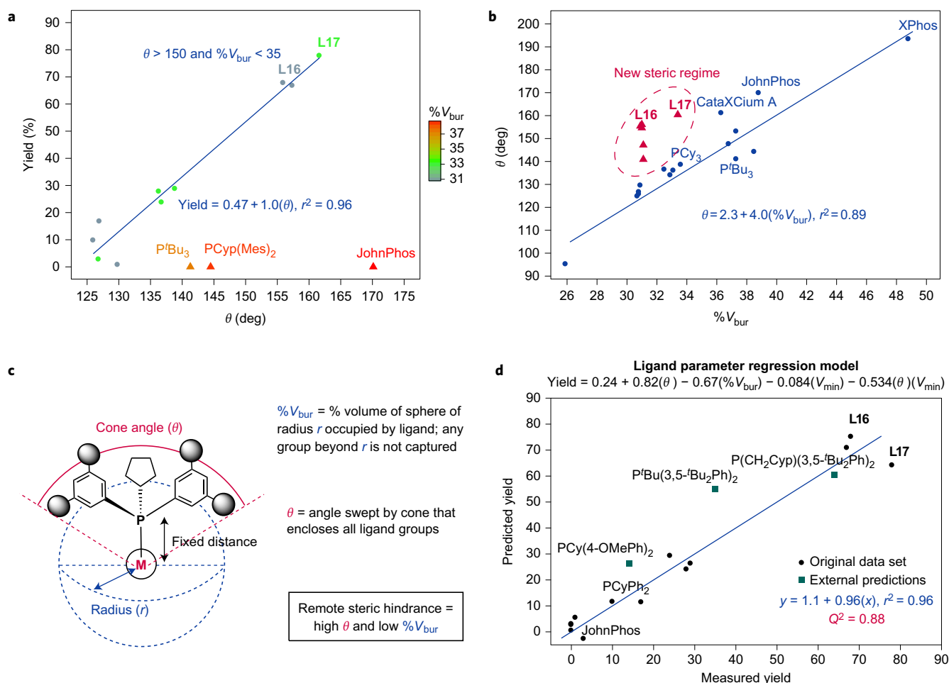
Figure 3 | Steric parameterization and analysis. a , Plot of yield versus cone angle ( \theta ) and buried volume ( \%V_{\text{bur}} ). A comparison of the ligand steric parameters against reaction yield reveals that larger cone angle correlates with higher yield (circles), with the exception of ligands featuring high buried volume (triangles). The regression equation only includes the circle data points. b , Plot of cone angle versus buried volume. Cone angle and buried volume have previously been treated as equivalent measures of ligand steric environment, as illustrated by a 1:1 mapping of the two parameters (circle data points). The new phosphines prepared in this study (triangles) fall outside this 1:1 mapping, highlighting that these two terms are not equivalent, by definition. c , Definition of cone angle and buried volume. Both measure steric encumbrance but with different distance dependencies. Buried volume only accounts for steric hindrance proximal to the metal whereas cone angle is sensitive to ligand size at a distance. A ligand with a large cone angle and low \%V_{\text{bur}} , such as those most successful in this new method, therefore possesses remote steric hindrance. d , Plot of predicted yield versus actual yield. A quantitative model to relate cone angle, buried volume and V_{\text{min}} to yield was obtained by regression analysis. This model accounts for the entire scope of ligands tested in the study and features a mathematical representation of the remote steric effect concept. We show that the model can predict the performance of ligands (green squares) that feature unique structural motifs to those included in the ligand training set.
