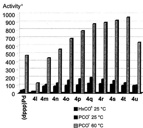
Fig. 5. Catalytic activity in the 1-alkene/CO copolymerization in \text{CH}_2\text{Cl}_2 . *Activity in (\text{g polymer}) \times (\text{g Pd} \times \text{h})^{-1} . b 1-Hexene/CO polymerization. c Propene/CO copolymerization.
