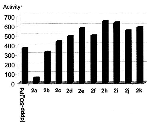
Fig. 4. Catalytic activity in the ethene/CO copolymerization in water. a Activity in (g polymer) \times (g Pd \times h) -1 .
