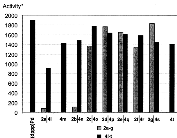
Fig. 3. Catalytic activity in the ethene/CO copolymerization in methanol. a Activity in (g polymer) \times (g Pd \times h) -1 .
