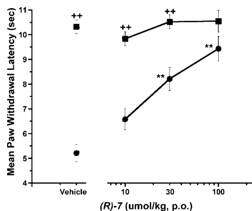
Figure 2. ( R )-7 has full efficacy against acute inflammatory thermal hyperalgesia induced by intraplantar carrageenan in the rat. Circles represent paw withdrawal latencies ipsilateral to the injury; squares represent paw withdrawal latencies contralateral to the injury. Data represent mean ± SEM [ F (7,95) = 26.61, p < 0.0001]. ** p < 0.01, as compared to vehicle-treated animals. ++ p < 0.01, as compared to carrageenan-treated paw ( n = 12 per group).
