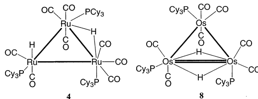
Fig. 4. Proposed structure of the 48\text{ e}^- cluster \text{H}_2\text{Ru}_3((\text{CO})_8(\text{PCy}_3)_3) ( 4 ) and structural plot of the 46\text{ e}^- cluster \text{H}_2\text{Os}_3((\text{CO})_7(\text{PCy}_3)_3) ( 8 ).
