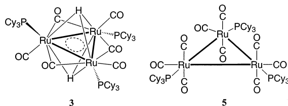
Fig. 1. Structural plots of the 44 e − \text{H}_2\text{Ru}_3((\text{CO})_6(\text{PCy}_3)_3 ( 3 ) and the 48 e − cluster \text{Ru}_3((\text{CO})_9(\text{PCy}_3)_3 ( 5 ).
