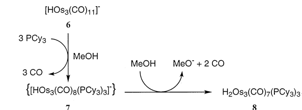
Scheme 2. Reaction of [\text{H}_2\text{Os}_3(\text{CO})_{11}]^- ( 6 ) with \text{PCy}_3 in methanol. The intermediate 7 is hypothetical.
