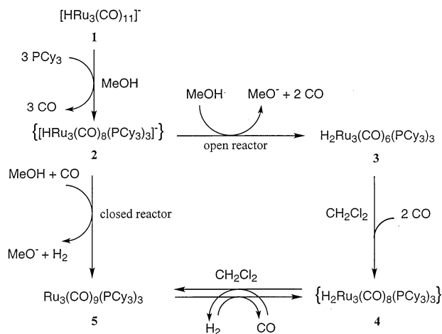
Scheme 1. Reaction of [\text{HRu}_3(\text{CO})_{11}]^- ( 1 ) with \text{PCy}_3 in methanol. The intermediate 4 is characterised in solution, species 2 is hypothetical.
