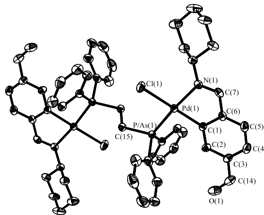
Fig. 1. Molecular structure of [\{\text{Pd}[4-(\text{COH})\text{C}_6\text{H}_3\text{C}(\text{H})=\text{N}(\text{Cy})-\text{C2},\text{N}](\text{Cl})\}_2(\mu-\text{Ph}_2\text{PCH}_2\text{CH}_2\text{AsPh}_2)] ( 2 ), with labeling scheme. Hydrogen atoms have been omitted for clarity.
