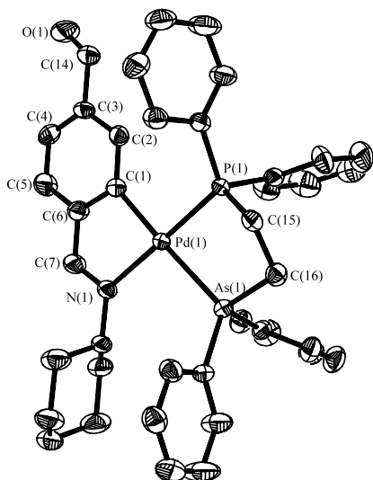
Fig. 2. Molecular structure of the cation for [\text{Pd}\{4\text{-(COH)C}_6\text{H}_3\text{C(H)=N(Cy)-C2,N}\}\{\text{Ph}_2\text{PCH}_2\text{CH}_2\text{AsPh}_2\text{-P,As}\}][\text{PF}_6] ( 3 ), with labeling scheme. Hydrogen atoms have been omitted for clarity.
