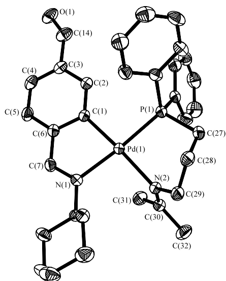
Fig. 3. Molecular structure of the cation for [\text{Pd}\{4\text{-(COH)C}_6\text{H}_3\text{C(H)=N(Cy)-C2,N}\}\{\text{Ph}_2\text{PCH}_2\text{CH}_2\text{CH}_2\text{N(=CMe}_2\text{)-P,N}\}][\text{PF}_6] ( 4 ), with labeling scheme. Hydrogen atoms have been omitted for clarity.
