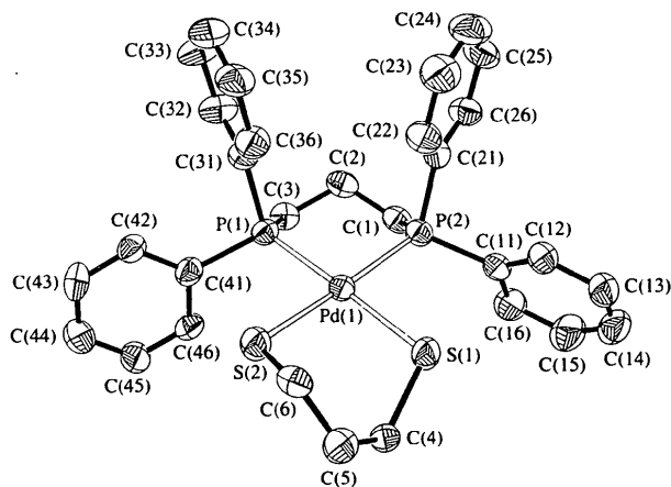
Fig. 1. The crystal structure of the title complex with ellipsoids drawn at the 30% probability level.
