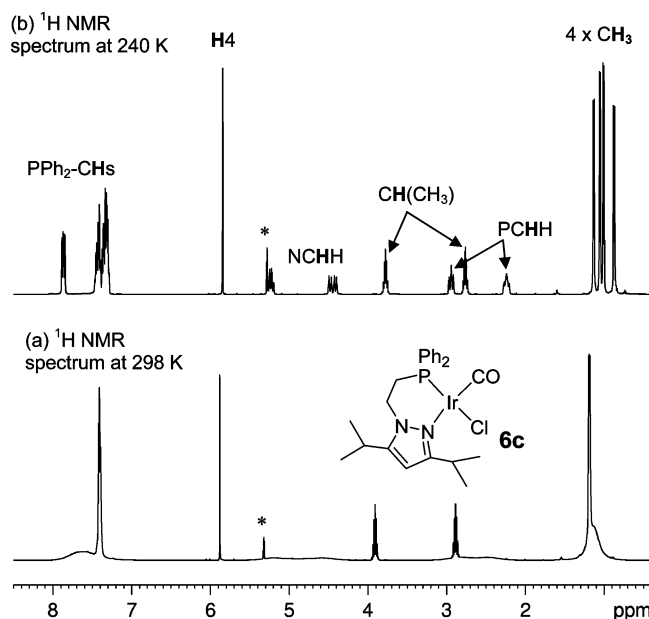
Figure 3. ^1\text{H} NMR spectra (500 MHz, \text{CD}_2\text{Cl}_2 ) of [\text{Ir}(i\text{Pr}_2\text{PyP})(\text{CO})\text{Cl}] ( 6c ) at (a) 298 K and (b) 240 K (* denotes the residual solvent resonance).
