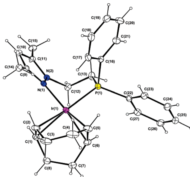
Figure 1. ORTEP depiction of the cationic fragment of [Ir(Me 2 PyP)(COD)]BPh 4 ( 3b ) at 20% thermal ellipsoids for the non-hydrogen atoms. Selected bond lengths (Å) and angles (deg): Ir(1)–P(1) = 2.2882(6); Ir(1)–N(1) = 2.1045(16); Ir(1)–C(1) = 2.2072(2); Ir(1)–C(2) = 2.33(2); Ir(1)–C(5) = 2.132(7); Ir(1)–C(6) = 2.140(2); C(1)–C(2) = 1.379(3); C(5)–C(6) = 1.408(3); P(1)–Ir(1)–N(1) = 84.31(5); P(1)–Ir(1)–C(5) = 93.73(7); P(1)–Ir(1)–C(6) = 95.99(6); N(1)–Ir(1)–C(1) = 91.43(7); N(1)–Ir(1)–C(2) = 96.69(8); C(1)–Ir(1)–C(6) = 81.05(8); C(2)–Ir(1)–C(5) = 80.62(10); C(1)–Ir(1)–C(5) = 96.92(9); C(2)–Ir(1)–C(6) = 87.92(9).
