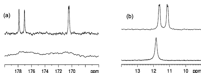
Figure 2. NMR spectra of [\text{Ir}(\text{PyP})(^{13}\text{CO})_2]\text{BPh}_4 ( 5a' ) in \text{CD}_2\text{Cl}_2 . (a) Carbonyl region of the ^{13}\text{C}\{^1\text{H}\} (125 MHz) spectra at 298 K (bottom) and 215 K (top); (b) ^{31}\text{P}\{^1\text{H}\} (202 MHz) spectra at 298 K (bottom) and 215 K (top).
