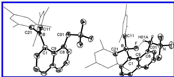
Figure 1. Crystal structure of one of the independent molecules of [3]^+ in [3][\text{OTf}] (left) and 3-F (right) (50% ellipsoid). Pertinent parameters are provided in the text.
