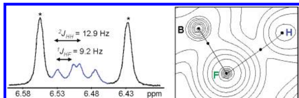
Figure 2. (left) Portion of the NMR showing the resonance of the hydrogen atom hydrogen-bonded to the fluorine atom. The peaks marked by * correspond to mesityl CH resonances; (right) contour plot of the electron density of 3-F in the B-F...H plane along with bond paths and bond critical points.
