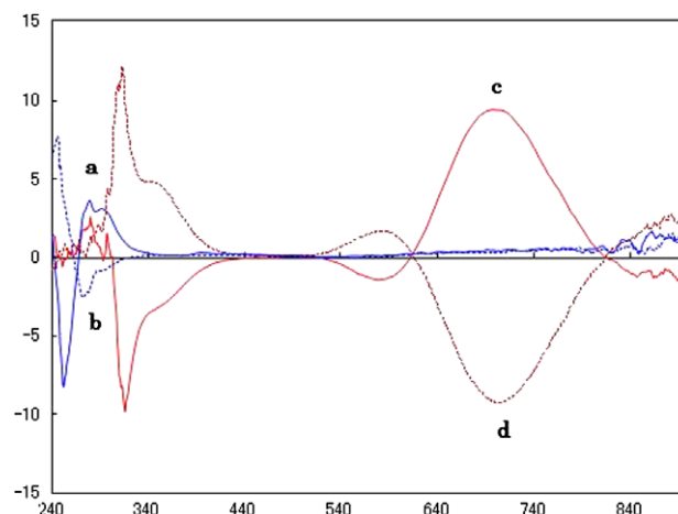
Fig. 1. CD spectra of (a) (+)- 1 , (b) (–)- 1 , (c) (+)- 1 –Cu(OAc) 2 complex, and (d) (–)- 1 –Cu(OAc) 2 complex in EtOH.
