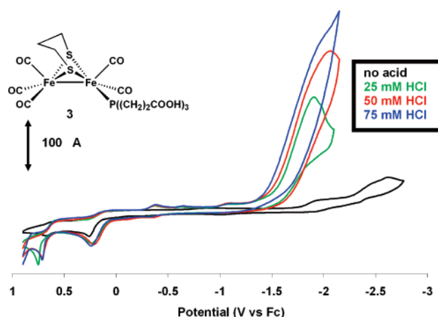
Figure 3. Cyclic voltammograms of 3 (2.5 mM in 0.1 M t\text{Bu}_4\text{NBF}_4 in MeCN under Ar) with increments of HCl (0, 25, 50, and 75 mM).
