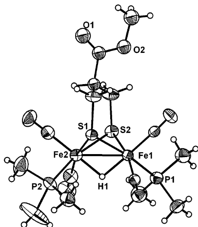
Figure 7. Thermal ellipsoid representation (50% probability) of \{(\mu-(\text{SCH}_2)_2\text{CHCOMe})(\mu\text{-H})[\text{Fe}(\text{CO})_2(\text{PMe}_3)_2]_2\}\text{PF}_6 ( 6 ). The \text{PF}_6^- counteranion has been omitted.
