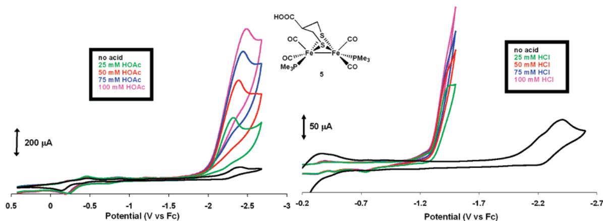
Figure 4. Cyclic voltammograms of 5 (MeCN, 0.1 M t\text{BuNBF}_4 ) in the presence of 0, 25, 50, 75, and 100 mM HOAc (left) and HCl (right).
