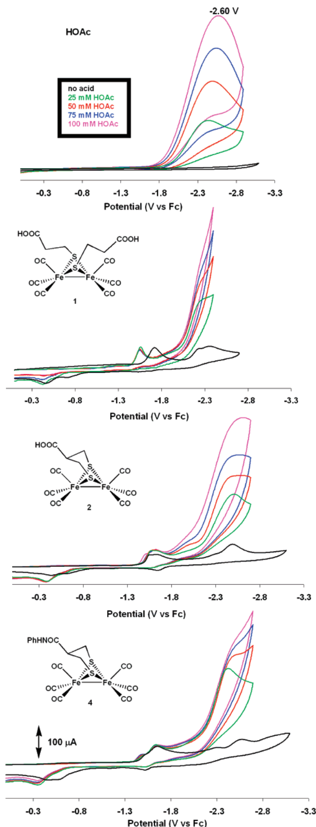
Figure 2. Cyclic voltammograms of complexes 1 , 2 , and 4 (2.5 mM) with HOAc (0, 25, 50, 75, 100 mM) in 0.1 M t\text{Bu}_4\text{NBF}_4 in CO-saturated \text{CH}_3\text{CN} . The CV of HOAc in MeCN at these concentrations is shown as a control.
