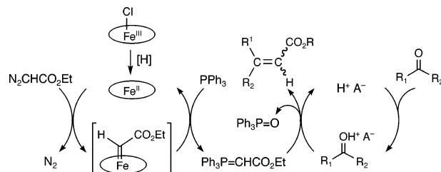
Scheme 1. Possible Mechanism for Acid-Promoted Olefination of Ketones by Fe(TPP)Cl
