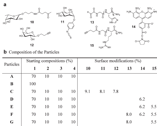
Figure 2. Modules for surface modification and chemical composition of nanoparticles. The chemical structures of compounds 10–15 used for surface modification of the nanoparticles (a). The chemical compositions of the various nanoparticles (b).
