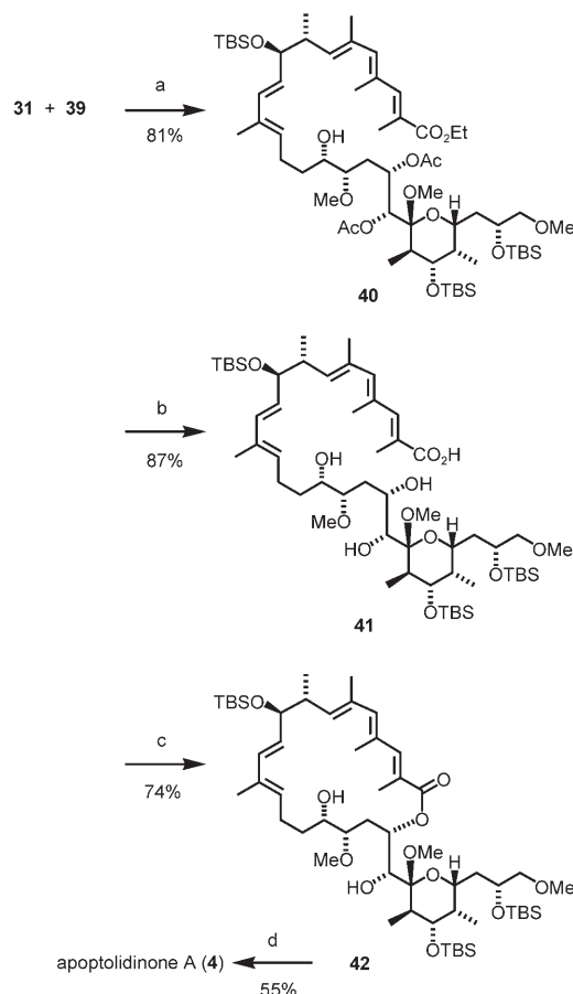
Scheme 7. a) Cu I -thiophene-2-carboxylate, N -methylpyrrolidinone, −10 °C; b) LiOH, THF/MeOH/H 2 O, 40 °C; c) 2,4,6-trichlorobenzoyl chloride, Et 3 N, THF, 25 °C, then DMAP, toluene, 80 °C; d) HF-pyridine, THF, 0 → 25 °C.
