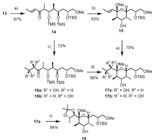
Scheme 3. a) ( E )-1-bromo-1-propene, t BuLi, Et 2 O, –78 °C; b) PPTS, MeOH, CH 2 Cl 2 , 0 °C; c) AD-mix \alpha , t BuOH/H 2 O, 0 °C, 16a/16b 3:1; d) PPTS, MeOH, CH 2 Cl 2 , 0 °C; e) [K 2 OsO 2 (OH) 4 ], NMO, THF/H 2 O/ t BuOH, 20 °C; f) 2,2-dimethoxypropane, CSA, 0 °C. PPTS = pyridinium p -toluenesulfonate, NMO = N -methylmorpholine- N -oxide, CSA = camphorsulfonic acid.
