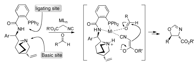
Scheme 2. Postulated Catalyst Activation Mode
