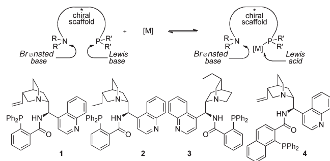
Scheme 1. Cooperative Catalysis Concept from Amino-phosphines and Metal Ions and a Library of Cinchona-Derived Precatalysts
