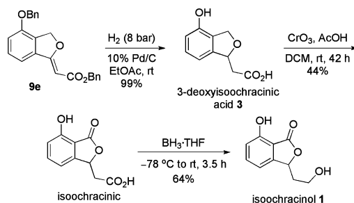
Scheme 4. Syntheses of the Natural Products 3-Deoxyisoochracinic Acid, Isochracinic Acid, and Isochracinol
