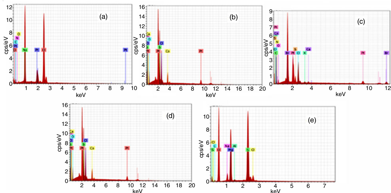
Fig. 3. FESEM spectra of (a) SM-31, (b) SM-36, (c) SM-37, (d) SM-16, (e) SM-27
