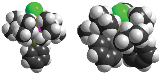
Figure 4. Space-filling models of [\text{PhBP}^{\text{iPr}}_3]\text{FeCl} (left) and [\text{SiP}^{\text{iPr}}_3]\text{FeCl} ( 6 ; right); [\text{PhBP}^{\text{iPr}}_3] = [\text{PhB}(\text{CH}_2\text{P}^{\text{iPr}}_2)_3]^- .
