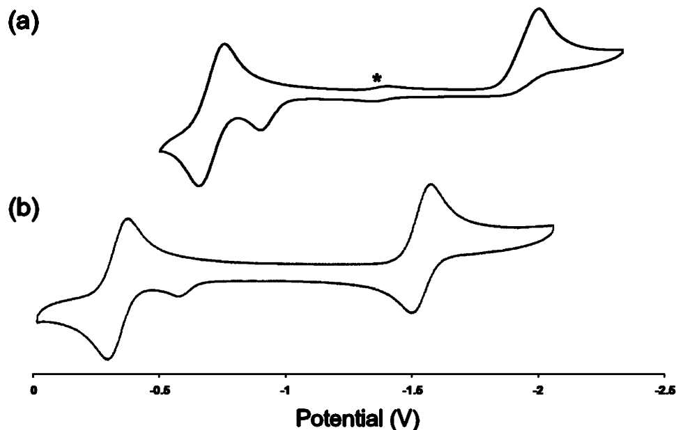
Figure 6. Cyclic voltammograms of (a) [\text{SiP}^{\text{iPr}}_3]\text{CoCl} ( 2 ) and (b) [\text{SiP}^{\text{Ph}}_3]\text{CoCl} ( 9 ) recorded at a scan rate of 100 mV/s (* denotes a trace impurity in 2 ). Both scans were recorded in THF under an \text{N}_2 atmosphere. Potentials are referenced to \text{Fc}/\text{Fc}^+ .
