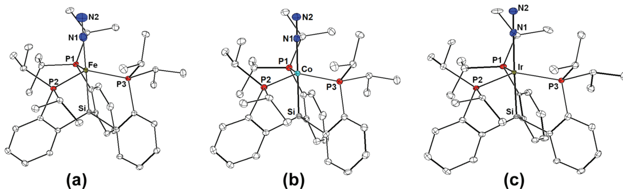
Figure 7. Displacement ellipsoid (35%) representations of (a) [\text{SiP}^{\text{iPr}}_3]\text{Fe}(\text{N}_2) ( 10 ), 26 (b) [\text{SiP}^{\text{iPr}}_3]\text{Co}(\text{N}_2) ( 12 ), and (c) [\text{SiP}^{\text{iPr}}_3]\text{Ir}(\text{N}_2) ( 14 ). Hydrogen atoms and solvent molecules have been omitted for clarity. Selected bond distances (Å) and angles (deg), for 10 : Fe–Si 2.2918(6), Fe–P1 2.3174(5), Fe–P2 2.2954(5), Fe–P3 2.3078(5), Fe–N1 1.817(4), N1–N2 1.065(5), P1–Fe–P2 115.14(1), P1–Fe–P3 119.18(2), P2–Fe–P3 117.82(2), Si–Fe–N1 178.83(6). For 12 : Co–Si 2.2327(6), Co–P1 2.2376(6), Co–P2 2.2277(6), Co–P3 2.2342(6), Co–N1 1.813(2), N1–N2 1.123(3), P1–Co–P2 117.48(2), P1–Co–P3 118.01(2), P2–Co–P3 119.51(2), Si–Co–N1 179.13(6). For 14 : Ir–Si 2.304(2), Ir–P1 2.336(2), Ir–P2 2.328(2), Ir–P3 2.315(2), Ir–N1 2.033(4), N1–N2 1.094(4), P1–Ir–P2 116.00(4), P1–Ir–P3 121.61(6), P2–Ir–P3 117.31(5), Si–Ir–N1 177.05(9).
