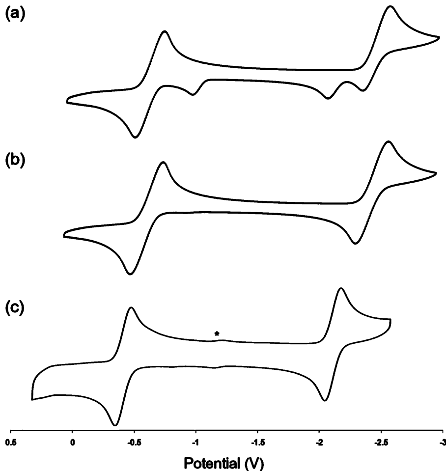
Figure 5. Cyclic voltammograms of (a) [\text{SiP}^{\text{iPr}}_3]\text{FeCl} ( 6 ) under \text{N}_2 , (b) [\text{SiP}^{\text{iPr}}_3]\text{FeCl} ( 6 ) under Ar, and (c) [\text{SiP}^{\text{Ph}}_3]\text{FeCl} ( 8 ) under \text{N}_2 (* denotes a trace impurity in 8 ). Scans (a) and (b) were recorded at a scan rate of 500 mV/s, and scan (c) was recorded at 100 mV/s. All data were acquired in THF and potentials are referenced to \text{Fc}/\text{Fc}^+ .
