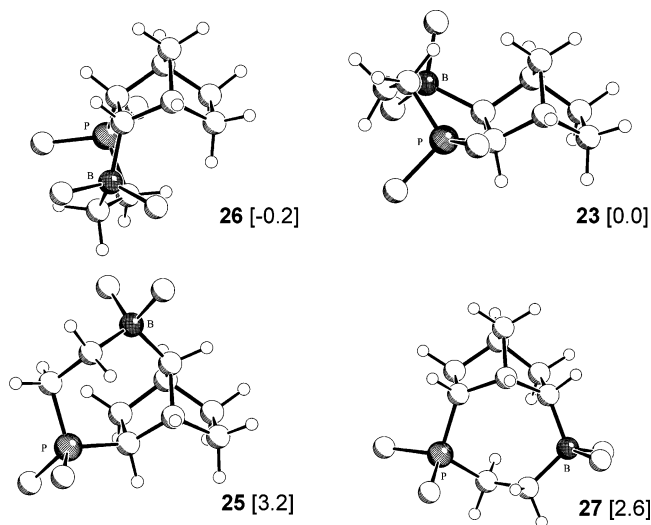
Figure 3. DFT-calculated structures and relative energies [in kcal mol −1 ] (B2PLYP-D/QZVP(-g,-f)//B97-D/def2-TZVP level) of the adducts 23 , 25 – 27 (for clarity, the major parts of the Mes and C 6 F 5 substituents are not shown).
