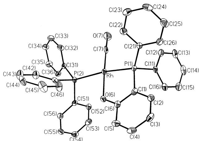
Fig. 3. Molecular structure of Rh(OC 6 H 4 PPh 2 )(CO)(PPh 3 ) (2).
