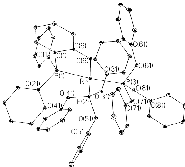
Fig. 4. Molecular structure of Rh(OC 6 H 4 PPh 2 ){P(OPh) 3 } 2 (3).
