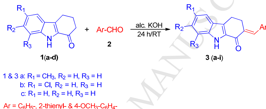
Scheme1. Synthesis of 2-arylidene/heteroliden-2,3,4,9-tetrahydrocarbazol-1-one 3
