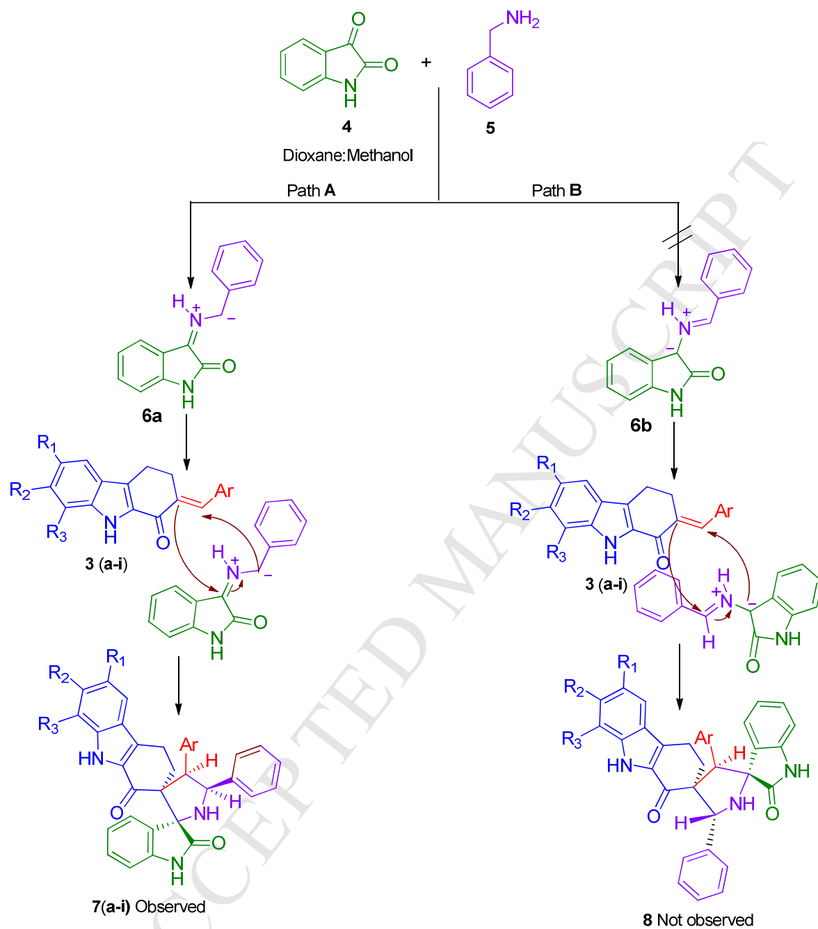
Scheme 3. Plausible the machanism for the formation of 7.
