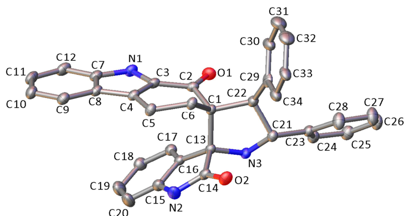
Figure 2. Structure of 7a with the atomic numbering scheme shown. Hydrogen atoms omitted and only one position of disorder phenyl ring (C29-C34) shown for clarity. Thermal ellipsoids depicted at the 50% probability level.
