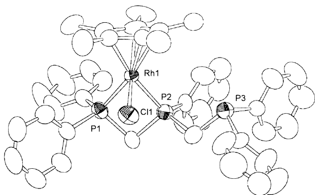
Fig. 1. Molecular structure of 2a(A) . A PF 6 was omitted for clarity. Selected bond lengths (Å) and angles (°): Rh(1)–Cl(1), 2.389(3); Rh(1)–P(1), 2.303(3); Rh(1)–P(2), 2.338(3); Cl(1)–Rh(1)–P(1), 83.9(1); Cl(1)–Rh(1)–P(2), 85.0(1); P(1)–Rh(1)–P(2), 71.6(1).
