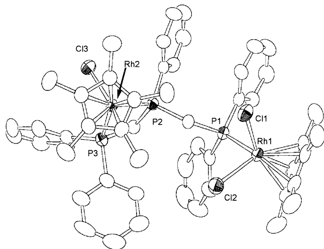
Fig. 2. Molecular structure of 3a(B) . A \text{PF}_6^- anion was omitted for clarity. Selected bond lengths (Å) and angles (°): Rh(1)–Cl(1), 2.420(2); Rh(1)–Cl(2), 2.425; Rh(1)–P(1), 2.335(2); Rh(2)–Cl(3), 2.375(2); Rh(2)–P(2), 2.314(2); Rh(2)–P(3), 2.305(2); Cl(1)–Rh(1)–Cl(2), 91.67(7); Cl(1)–Rh(1)–P(1), 88.64(5); Cl(2)–Rh(1)–P(1), 89.93(6); Rh(1)–P(1)–C(51), 106.9(2); P(1)–C(51)–P(2), 129.9(3); Cl(3)–Rh(2)–P(2), 86.02(5); Cl(3)–Rh(2)–P(3), 86.58(6); P(2)–Rh(2)–P(3), 72.28(5); Rh(2)–P(3)–C(52), 95.1(2); P(2)–C(52)–P(3), 95.78(3); Rh(2)–P(2)–C(52), 94.8(2).
