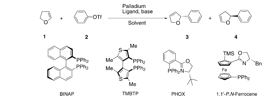
Scheme 1. The asymmetric intermolecular Heck reaction with 2,3-dihydrofuran and phenyl triflate.
