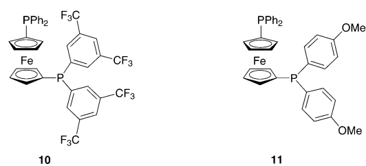
Scheme 7. The regioselectivities of Heck reaction catalyzed by ligands 10 and 11 with 1.5 mol % [\text{Pd}(\text{OAc})_2] in the presence of i\text{Pr}_2\text{NEt} and toluene at 60^\circ\text{C} .
