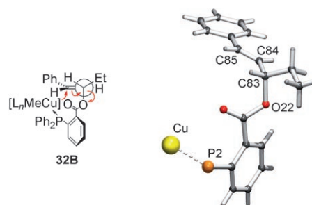
Figure 2. Postulated reactive conformation for the directed allylic substitution 32B and conformation of (–)-(E)-15 in the solid-state structure of copper complex 34 .
